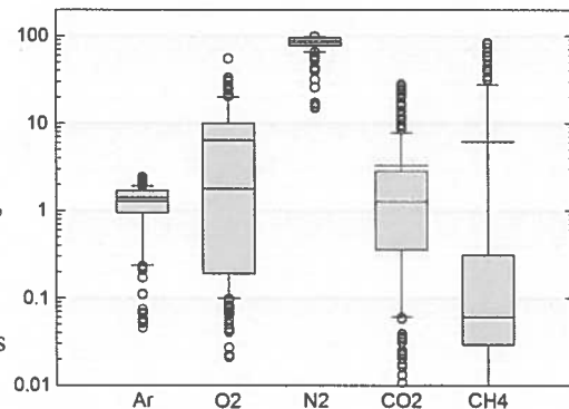
Figure 1: Box plot of composition of 277 gas samples, extracted from groundwater. Gray areas correspond to inter-quartiles, the black line is the median and the solid red line is the average. Atmospheric air samples and gas extracted from soil air show smaller variations and were not included in this plot.
