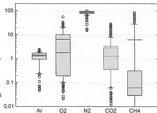
Figure 1: Box plot of composition of 277 gas samples, extracted from groundwater. Gray areas correspond to inter-quartiles, the black line is the median and the solid red line is the average. Atmospheric air samples and gas extracted from soil air show smaller variations and were not included in this plot.
