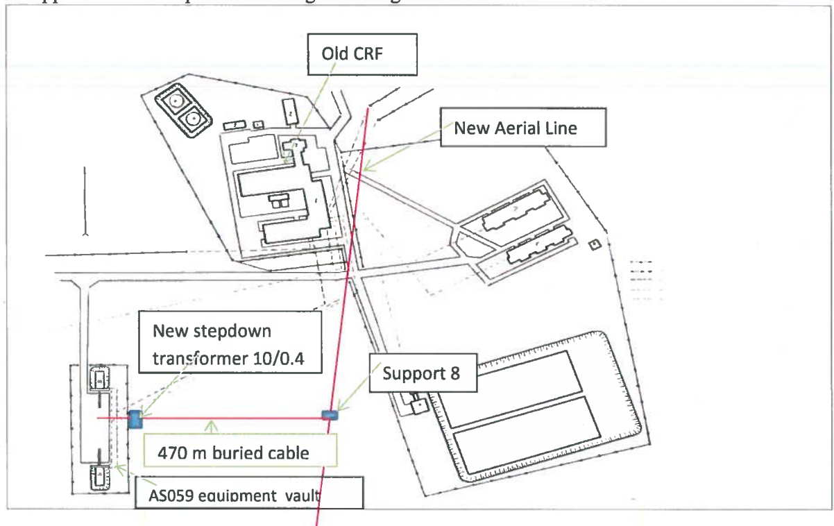
Figure 1. Layout of the new installation for the power connection to the equipment vault of AS059.
